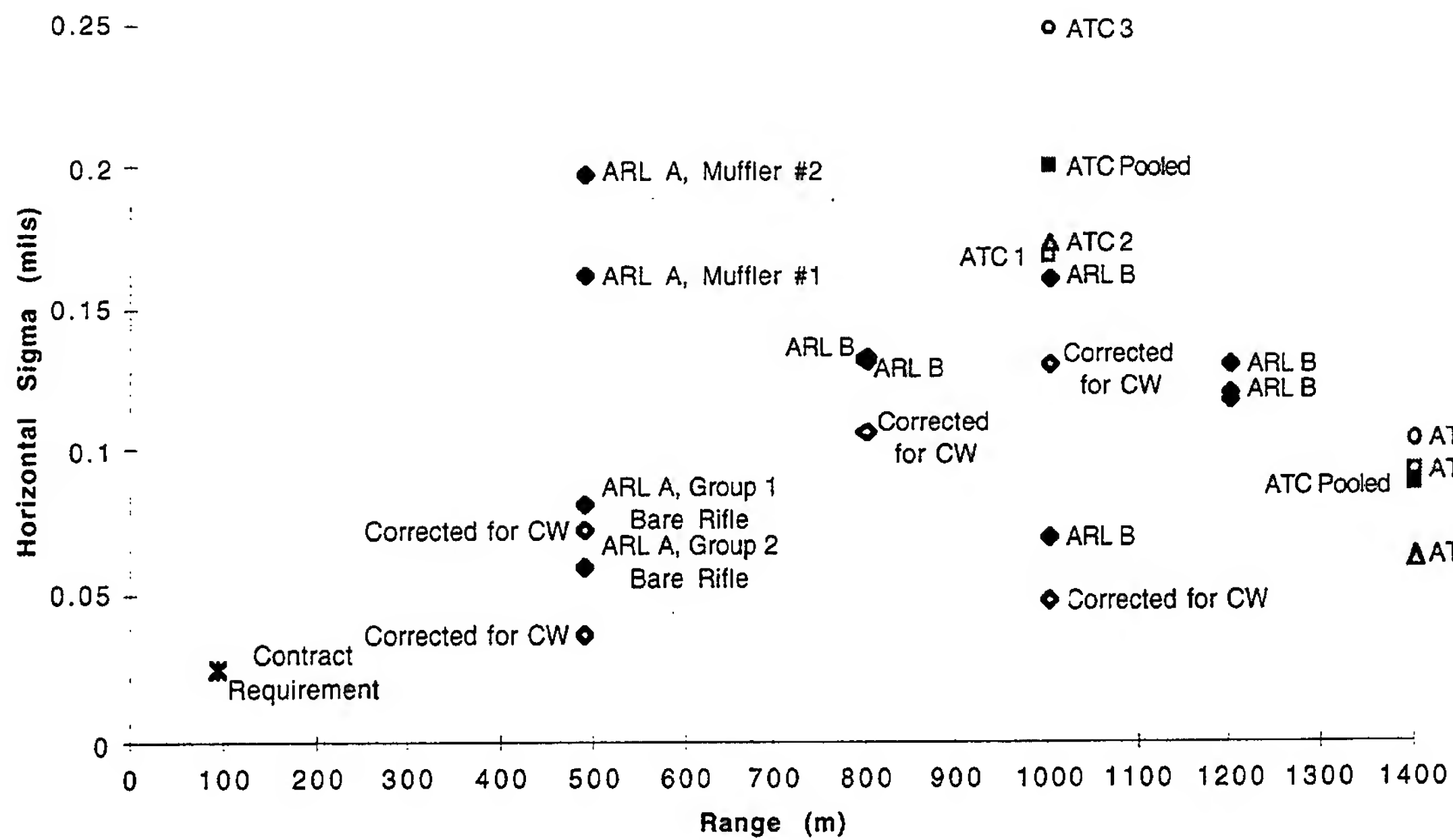
Figure A-3. Horizontal Dispersion Data, .338-.416.
